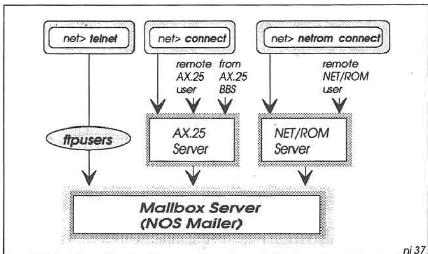
Fig 18-4: Logging in to a remote NOS BBS (using telnet or an ordinary AX.25 or NET/ROM connection).
